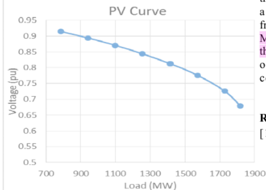
Figure 4.2 PV Curve
